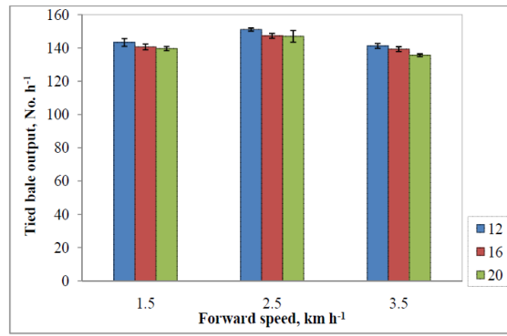
Fig. 4. Effect of forward speed of baler on output for without raking
