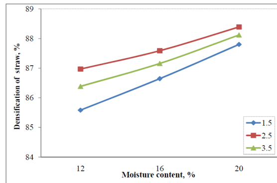
Fig. 8. Effect of moisture content of straw on densification of straw for with raking
